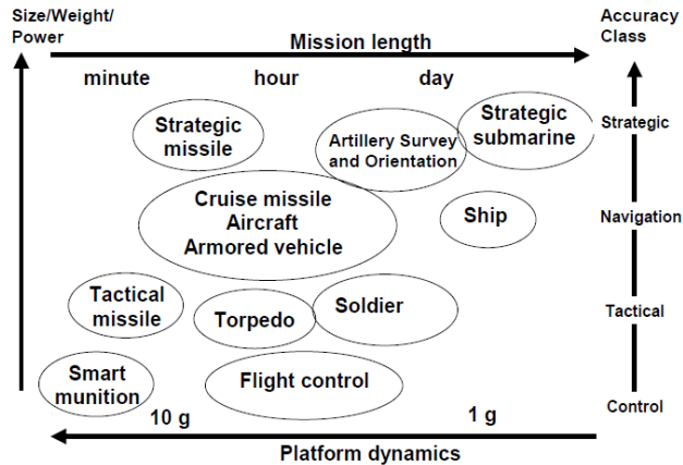
Figure 2 Classification and Usage Areas of Inertial Navigation Systems (NATO SET-054/RTG-30, 2004)
