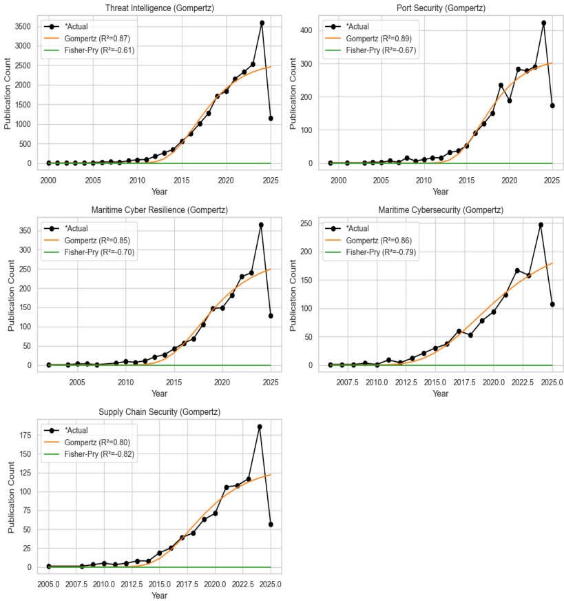
Figure 4 Growth Model Fit for Maritime Subdimension (Gompertz vs. Fisher - Pry)
