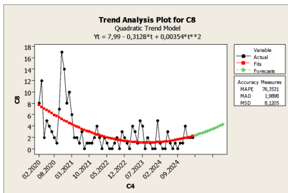
Figure 8 West Africa's Quadratic Trend Model of piracy
